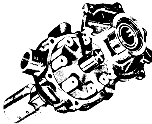
Figure 7-5. Roller pump.
